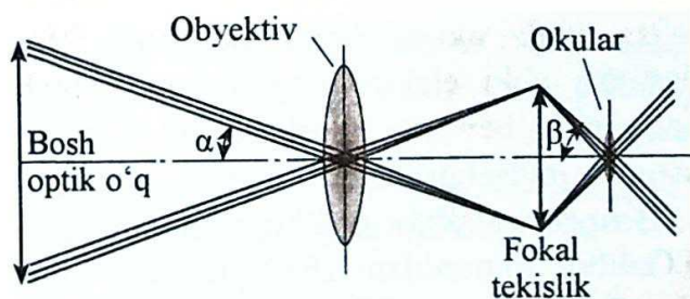
34-rasm. Linza teleskop (refraktor)ning tuzilishi (nurning yo'li).
