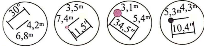
Saratonning \iota si Kassiopeya- ning \eta si Oqqushning \beta si Delfinning \gamma si
