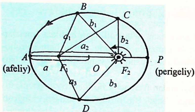
31-rasm. Planetaning ellips bo'ylab harakati.
