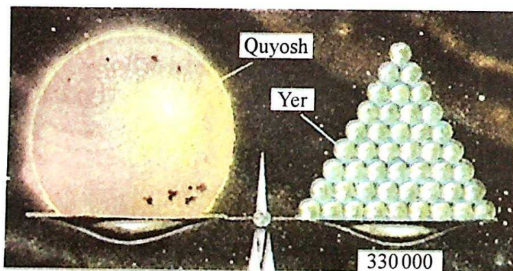
26-rasm. Yer massasini Quyosh massasi bilan solishtirish.
