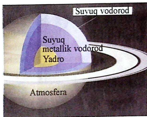
76-rasm. Saturnning ichki tuzilishi.
