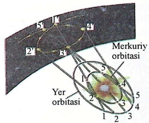
24-rasm. Planetalarning ko‘rinma sirtmoqsimon harakatini tushuntirish.
