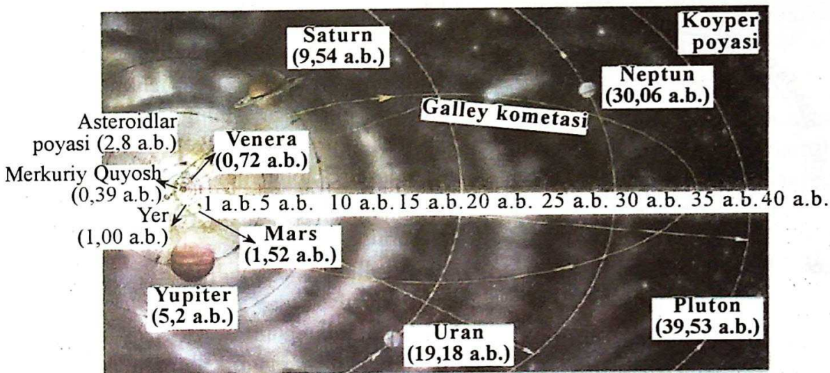
27-rasm. Quyosh sistemasining masshtabi (a.b. – astronomik birlik).
