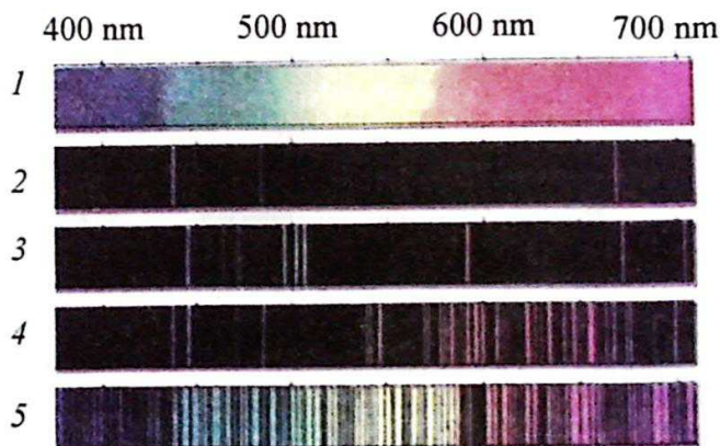
43-rasm. Yoritgichning tutash (1), solishtirish (2, 3, 4) va Quyoshning chiziqli (5) spektrlari.
